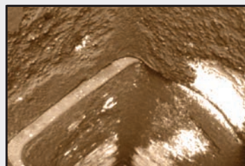
Actual photo of spalled flue tiles
