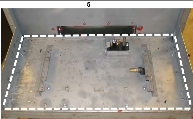
5. To remove entire Burner Pan, remove [16] DT Screws around perimeter of pan.
